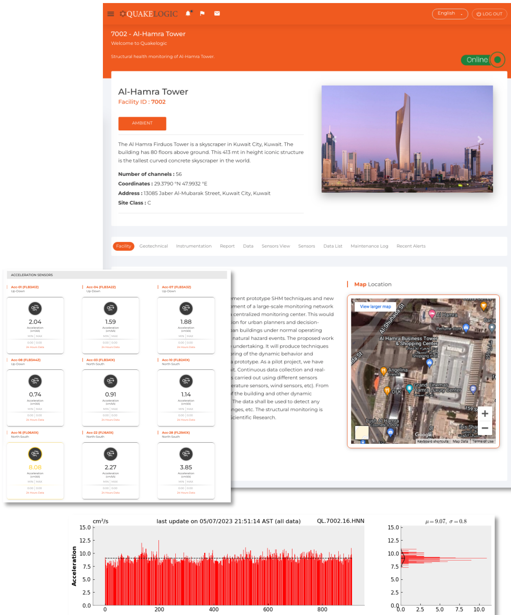
Figure 7. The SMARTBUILDING structural health monitoring dashboard overview for the Al-Hamra Tower.
